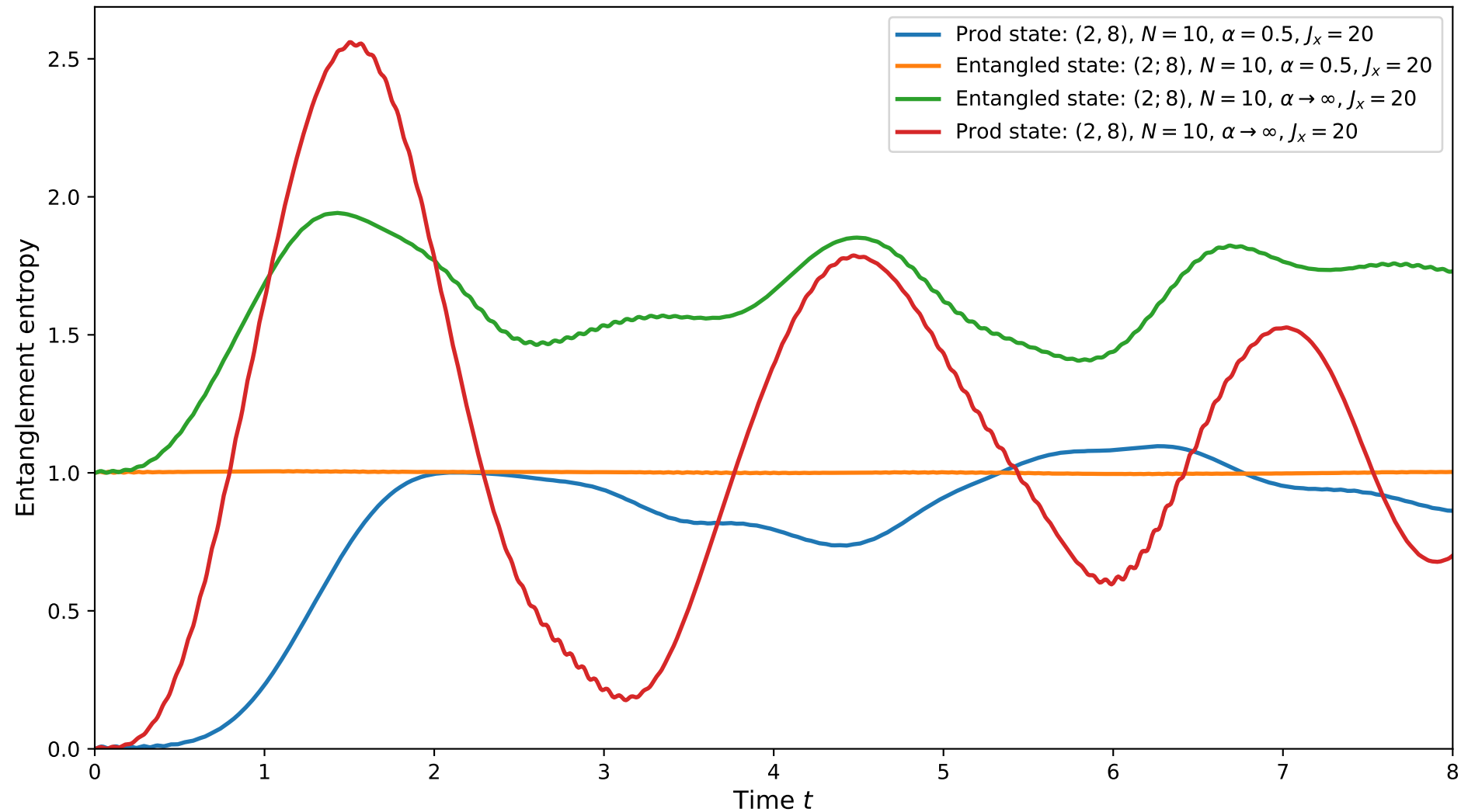
Time Evolution of Bipartite Entanglement Entropy
